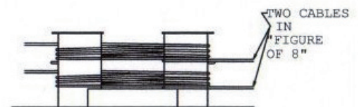
FIGURE C (EACH CABLE = 1/2 SWL) TWO CABLES IN "FIGURE OF 8" POSITIONED OVER UNDER THE SEPARATOR: EACH CABLE LOAD=1/2 SWL
